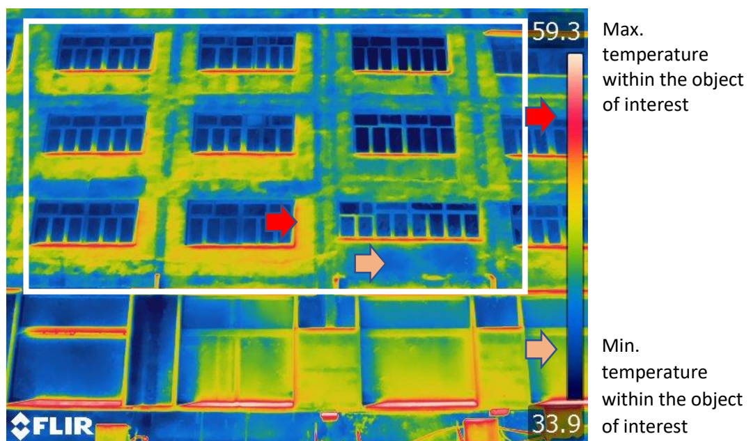
Figure 7 A thermogram satisfying the conditions required in Section 6.1.3 (fine weather condition), 6.3.5 (angle of incidence less than 40 deg), 6.3.9 (not more than four to five storeys) and 7.1 (maximum and minimum temperatures of the evenly/linearly distributed temperature bar in the object of interest highlighted in the white frame)
