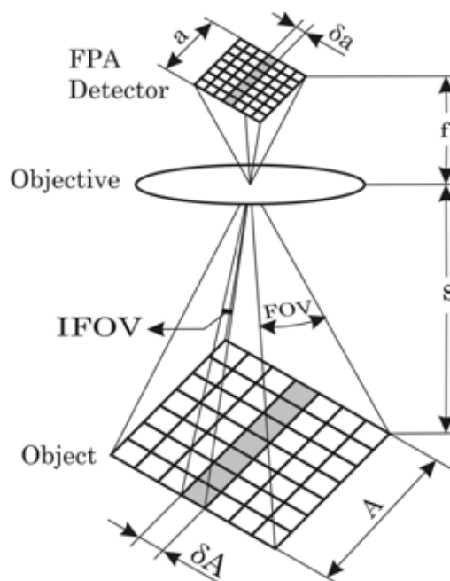
Figure 5 Definition of Instantaneous Field of View (IFOV) (Pencheva, Pulov, Gyoeh,
